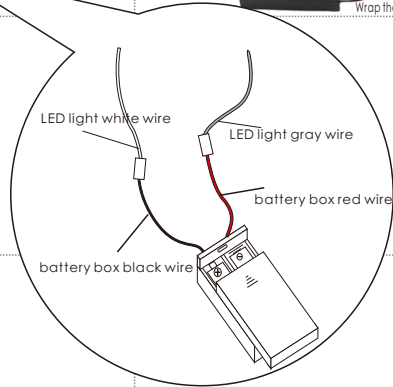
Wrap the exposed wires with H04
